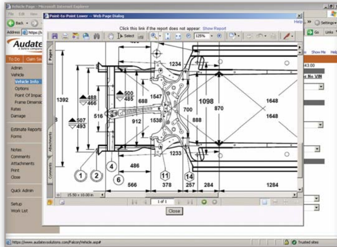
AUDATEX FRAME DIMENSIONS INCLUDES SPECIFICATIONS FOR POINT-TO-POINT, CENTERLINE AND DOOR OPENINGS
